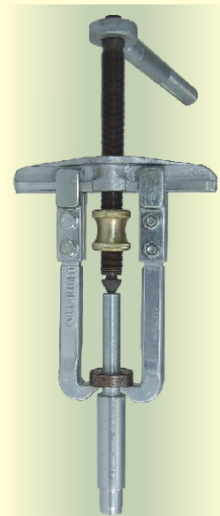
REMOVING BEARING
