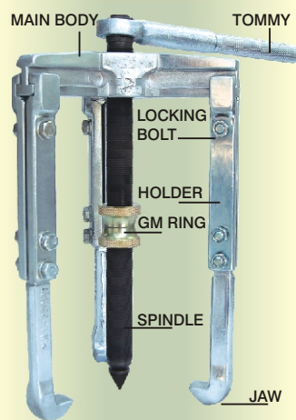
THREE JAW PULLER
